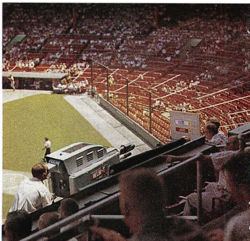
FIG. 2. Another multi-purpose color camera is located in a tv booth at third base. It performs a variety of assignments in both infield and outfield, and also picks up titles, such as running score.
