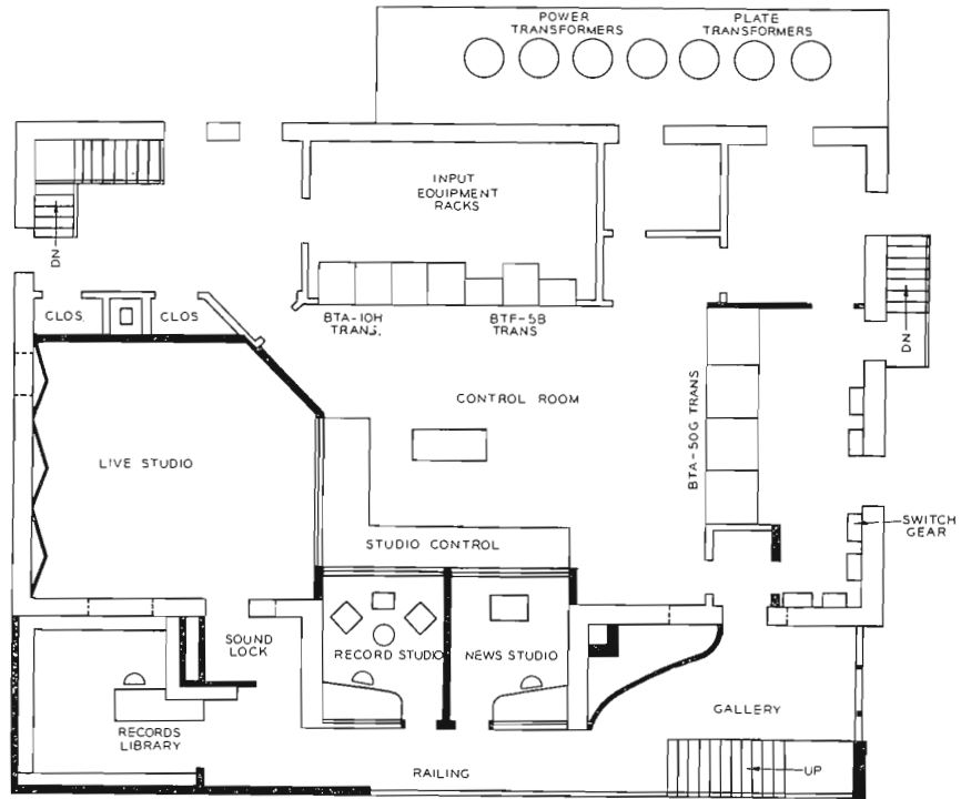
FIG. 2. All operating equipment is located in the large master control room. The three new transmitters are mounted along the walls at the side and rear of the room. Studio control positions are in front of each window with speech input equipment placed to the rear of the operating positions.
