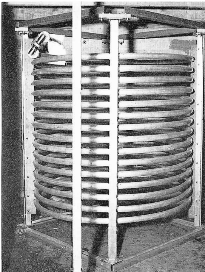
FIG. 9. This is the special FM isolation coil designed by the author. It is mounted in a separate building at the base of the center tower. This 52 by 71 inch coil is made from 1 \frac{3}{8} -inch Styroflex transmission line. The coil isolates the FM signal from the 30 kw AM signal on the tower.
