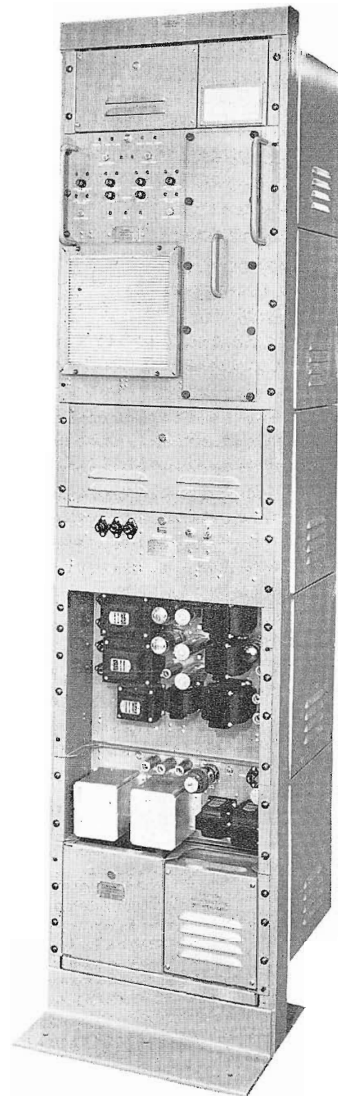
FIG. 1. The TVR-1 television satellite relay equipment designed by engineers of RCA Victor Company, Ltd., Montreal, to meet the needs of TV broadcasters desirous of extending their services to fringe or isolated areas.
