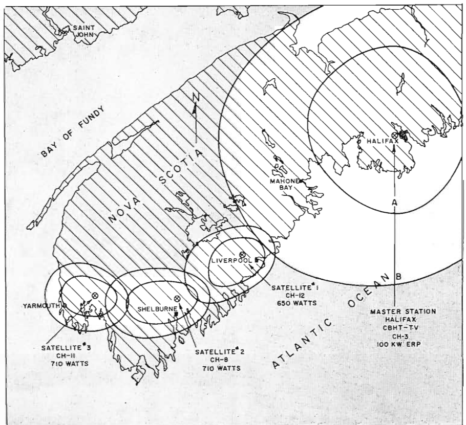
FIG. 6. Sketch of Nova Scotia illustrating extension of CBHT-TV coverage by three tandem satellites. (Contours are approximate only.)
