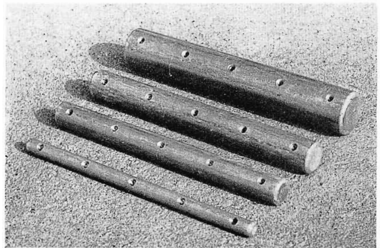
FIG. 6. This type of metal cylindrical coupler is used in UHF antennas. Its design permits adjustment of both phase and amplitude of the radiated field. Cylindrical coupling is mechanically simple, yet capable of handling high power.
