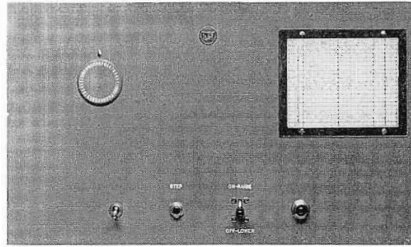
FIG. 5. This is the BTR-20A Transmitter Remote Control unit which performs all control functions on the BTA-1R Transmitter.
