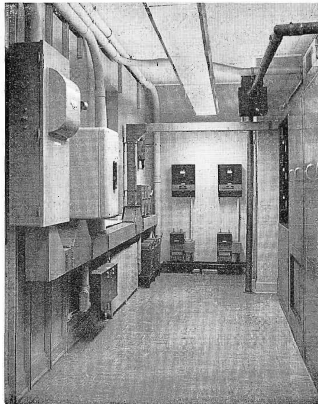
FIG. 4. Rear of the BTA-50G Transmitter. Note the ample access space provided for servicing the transmitter. The switch gear is conveniently mounted along the walls; and heavy distribution transformers on a floor supported platform. Mounting the transformers this way eliminated the need for reinforcing the walls.
