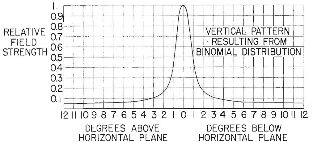
FIG. 13. A null-free pattern resulting from binomial distribution.
