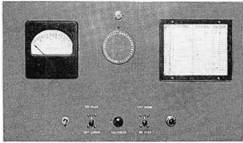
FIG. 2. This is the BTR-20 Studio Remote Control unit used at the WONA studios to control their BTA-1R transmitter on the outskirts of Winona.
